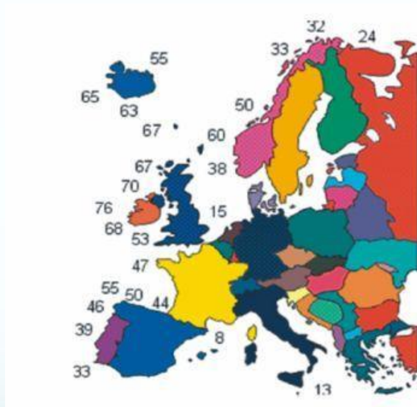
Europe: Average Annual Wave Power (kW/m) Courtesy of Sustainable Energy Authority of Ireland
